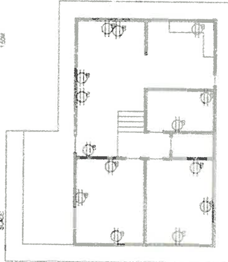
POWER LAYOUT PLAN
