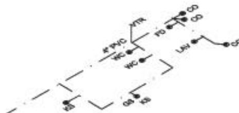
ISOMETRIC LAYOUT SEWAGE / DRAINAGE LINE LAYOUT PLAN SCALE: 1:100M
