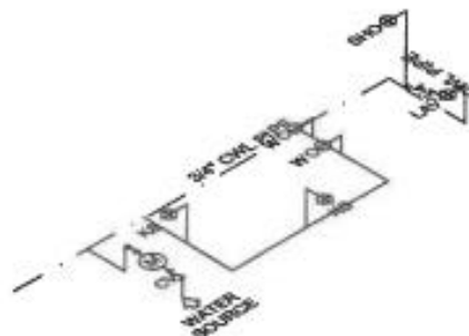
ISOMETRIC LAYOUT COLD WATER LINE LAYOUT SCALE: 1:100M
